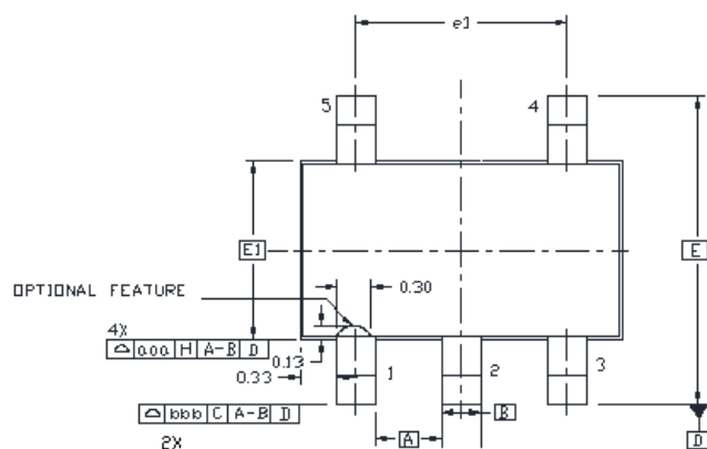
TOP VIEW 6 LEAD
