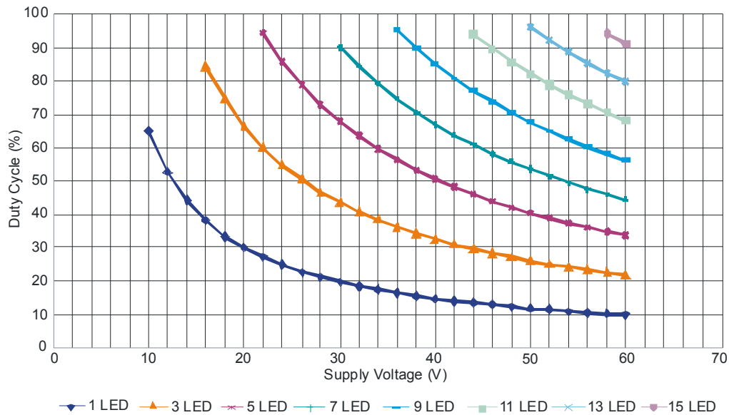
ZXLD1362 Duty Cycle L = 2200 \mu H
