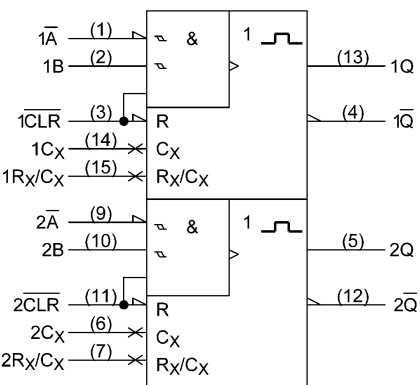
74VHC221AFT
