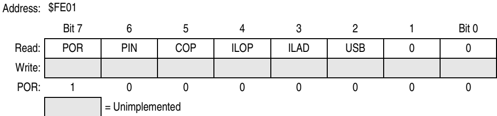
Figure 7-21. Reset Status Register (RSR)
