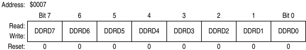
Figure 12-11. Data Direction Register D (DDRD)
