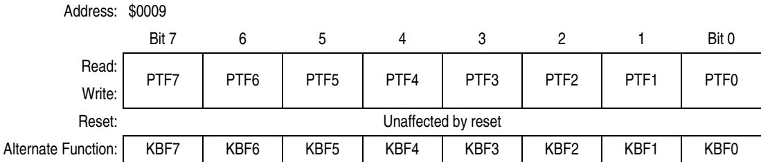
Figure 12-19. Port F Data Register (PTF)
