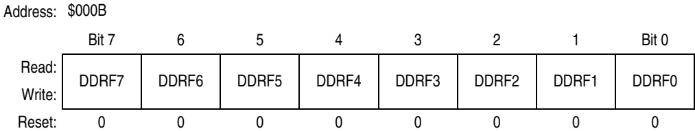
Figure 12-20. Data Direction Register F (DDRF)
