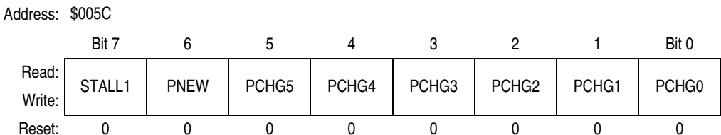
Figure 9-11. USB HUB Control Register 1 (HCR1)
