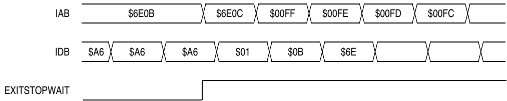
Figure 7-16. Wait Recovery from Interrupt or Break
