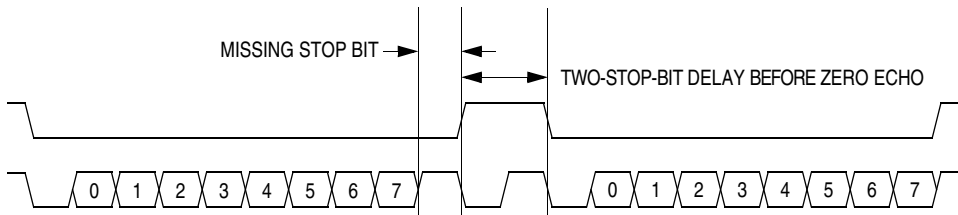
Figure 10-5. Break Transaction
