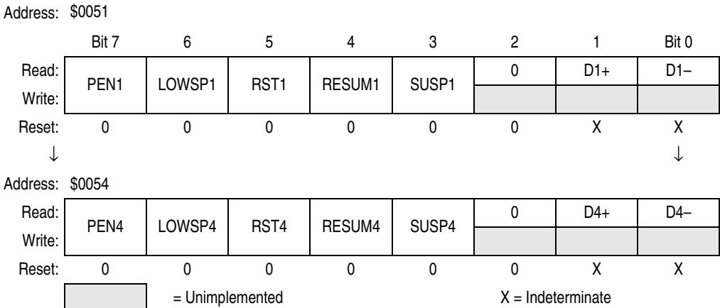
Figure 9-5. USB HUB Downstream Port Control Registers (HDP1CR-HDP4CR)
