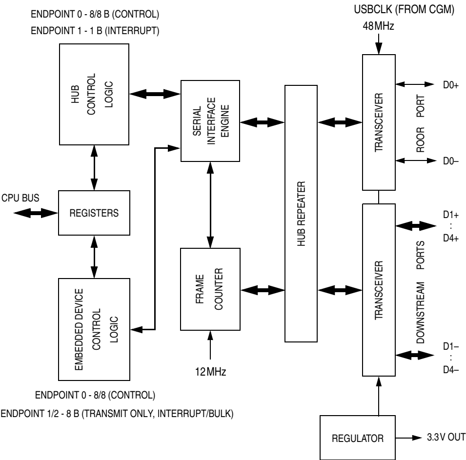
Figure 9-1. USB Block Diagram
