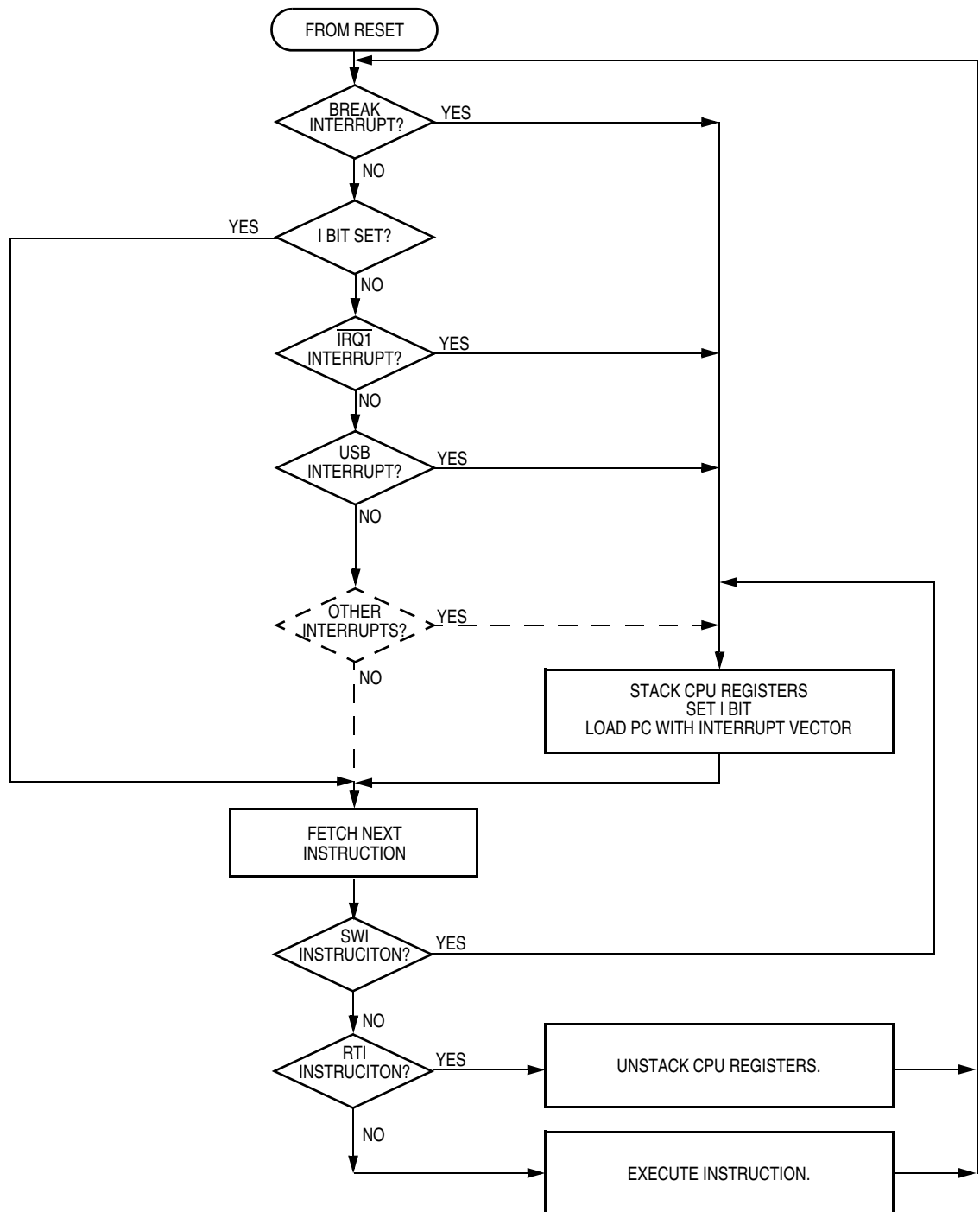
Figure 7-8. Interrupt Processing
