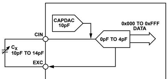
Figure 24. Using CAPDAC
