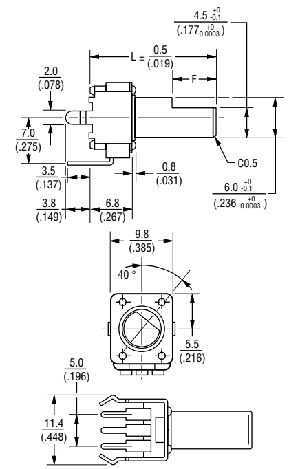
PTV09A-4 (with shaft style F)
