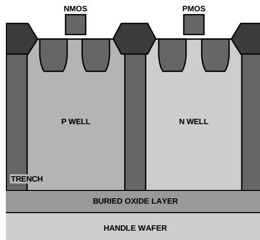
Figure 37. Trench Isolation
