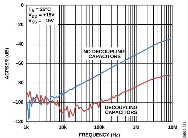
Figure 22. ACPSSR vs. Frequency, ±15 V Dual Supply
