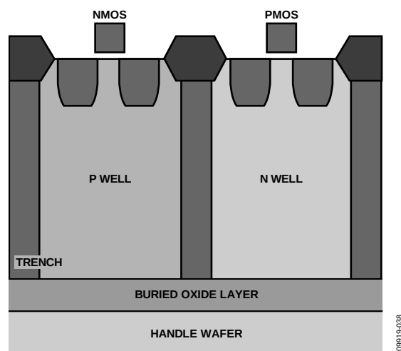
Figure 37. Trench Isolation
