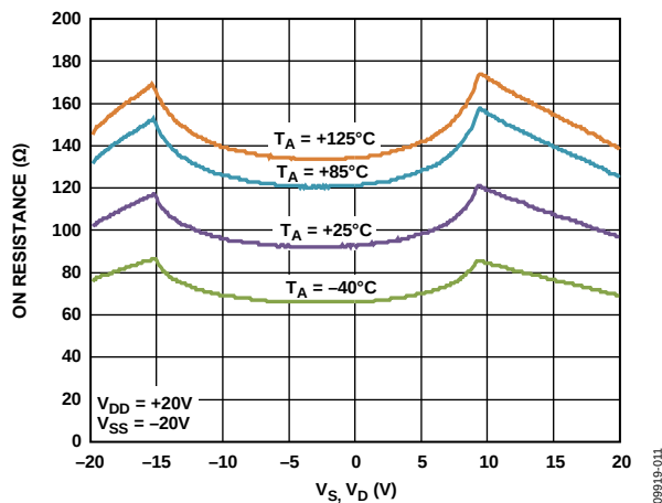
Figure 12. On Resistance as a Function of V_S (V_D) for Different Temperatures, \pm 20\text{ V} Dual Supply
