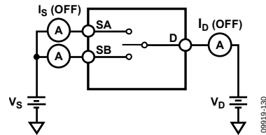
Figure 30. Off Leakage
