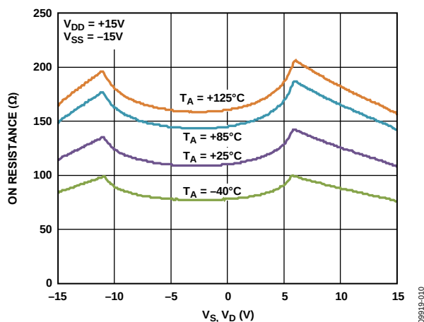
Figure 11. On Resistance as a Function of V_S (V_D) for Different Temperatures, \pm 15\text{ V} Dual Supply
