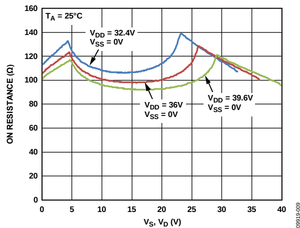
Figure 10. On Resistance as a Function of V_S, V_D (36 V Single Supply)
