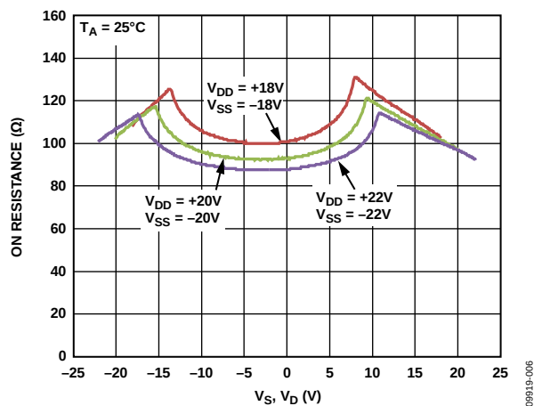
Figure 7. On Resistance as a Function of V_S, V_D ( \pm 20\text{ V} Dual Supply)
