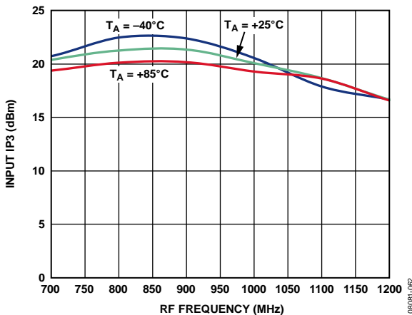
Figure 46. Input IP3 vs. RF Frequency at 3.3 V
