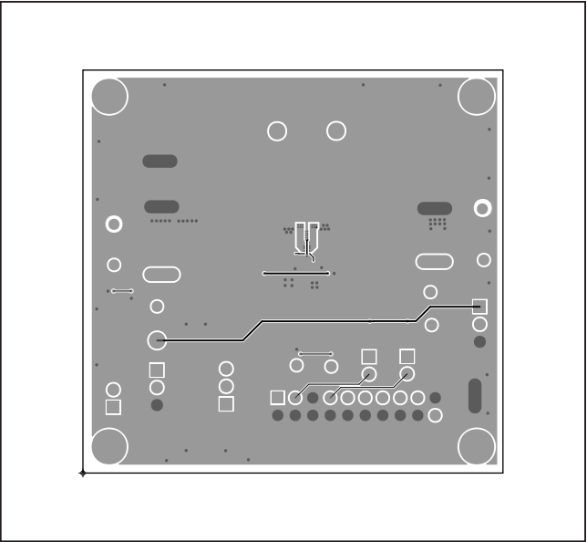
Figure 6. MAX8971 EV Kit PCB Layout—Top Side
