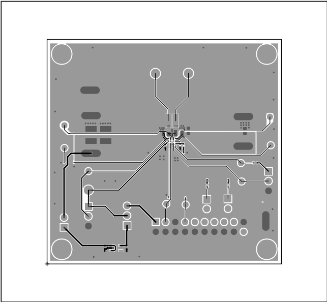
Figure 7. MAX8971 EV Kit PCB Layout—Bottom Side
