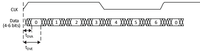
Figure 3.6.Receiver GDDR71_RX. Waveforms
