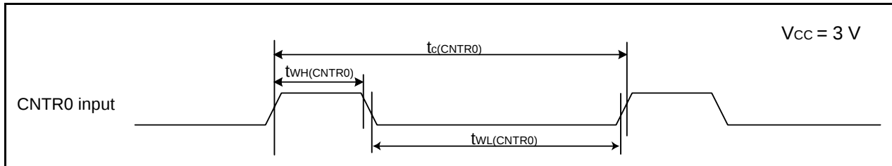
Figure 5.14 CNTR0 Input, CNTR1 Input, \overline{\text{INT1}} Input Timing Diagram when V_{CC} = 3\text{ V}
