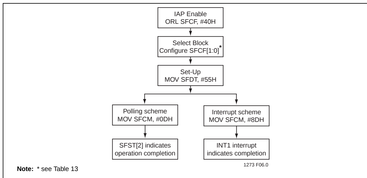
Figure 10: Block Erase
