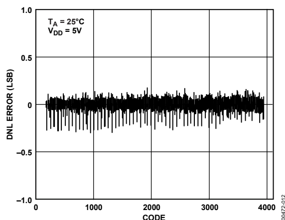
Figure 12. AD5323 Typical DNL Plot
