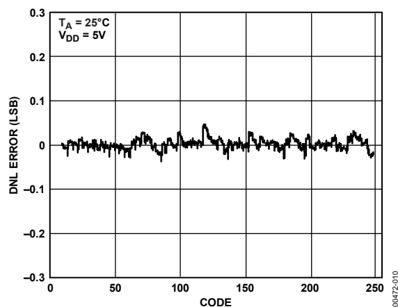
Figure 10. AD5303 Typical DNL Plot
