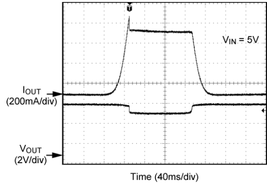
Figure 5. I OUT in Current Limiting for V OUT = 4V
