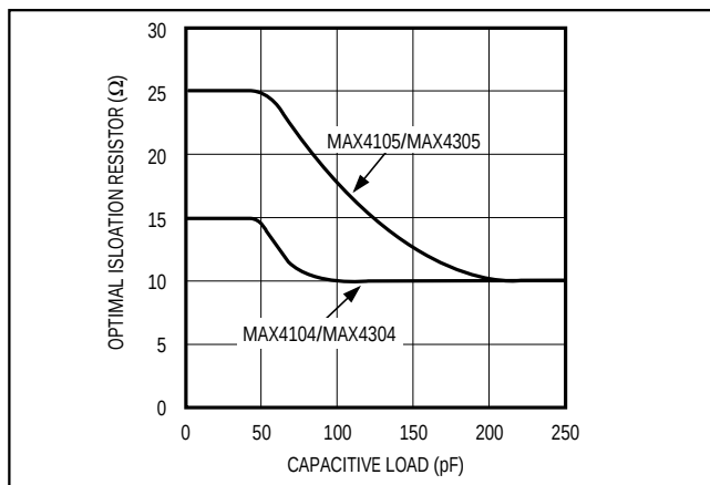
Figure 5. Optimal Isolation Resistor ( R_{ISO} ) vs. Capacitive Load
