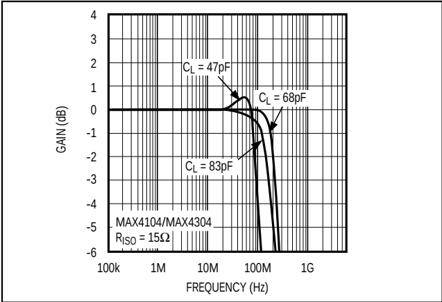
Figure 6. Frequency Responses vs. Capacitive Load with 15\Omega Isolation Resistor
