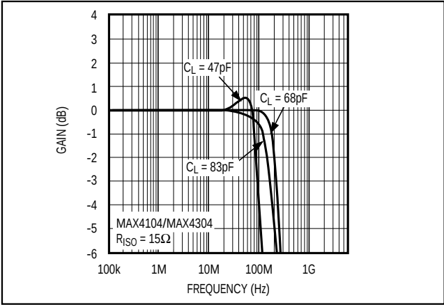
Figure 6. Frequency Responses vs. Capacitive Load with 15Ω Isolation Resistor
