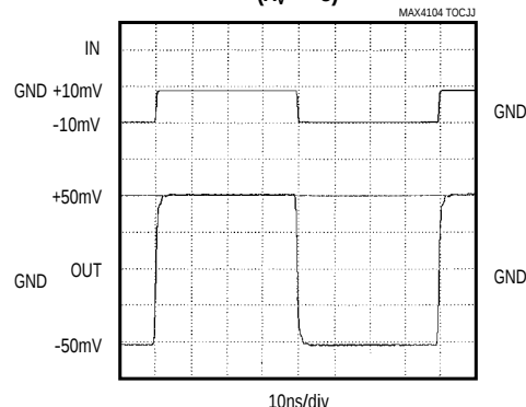
MAX4105 SMALL-SIGNAL PULSE RESPONSE ( A_V = +5 )
