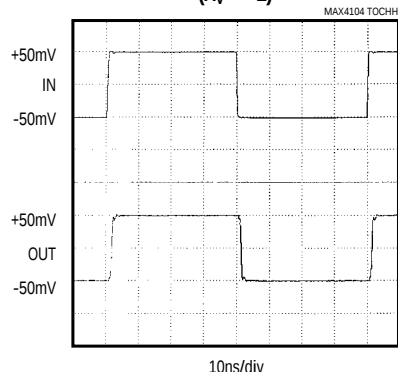
MAX4104 SMALL-SIGNAL PULSE RESPONSE ( A_V = +1 )
