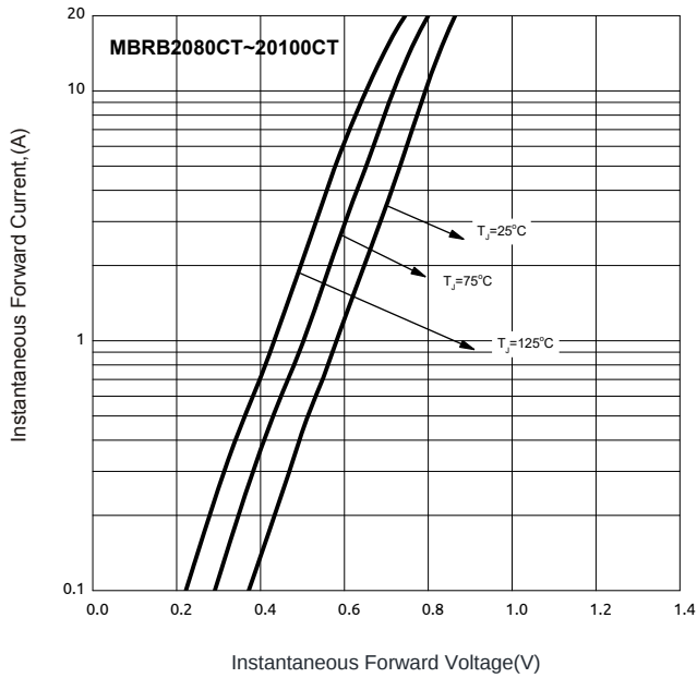
FIG.5-Typical Forward Characteristics
