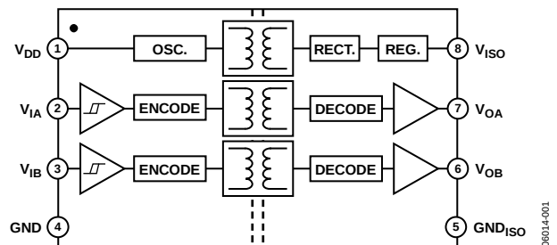
Figure 1. ADuM5240
