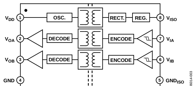
Figure 3. ADuM5242
