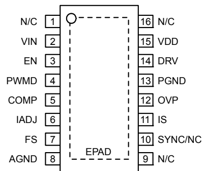
16-Pin TSSOP (TSE) MIC3230, MIC3231 See Product Option Matrix for selection
