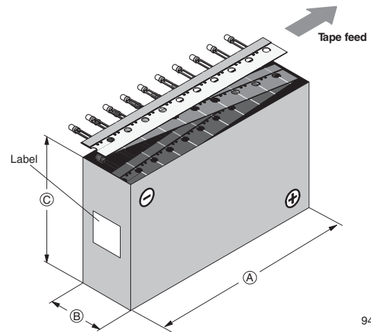
Fig. 41 - Tape Direction
