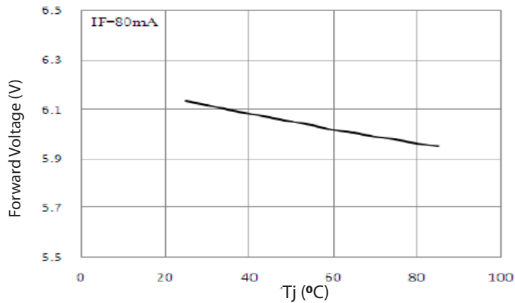
Tj--Forward Voltage
