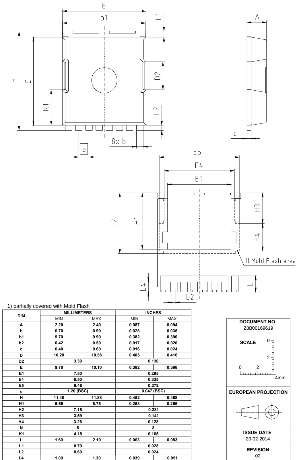
Figure 1 Outline PG-HSOF-8
