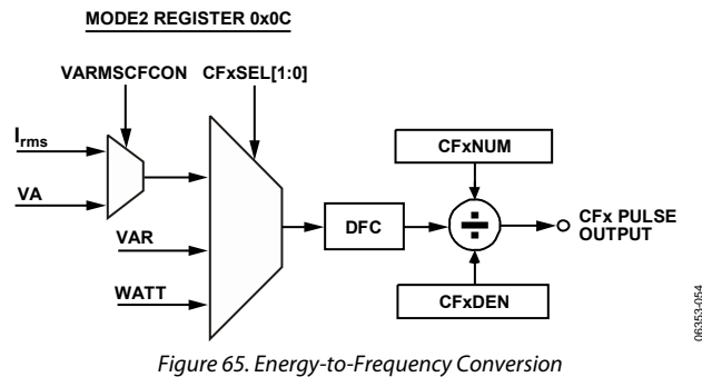
Figure 65. Energy-to-Frequency Conversion
