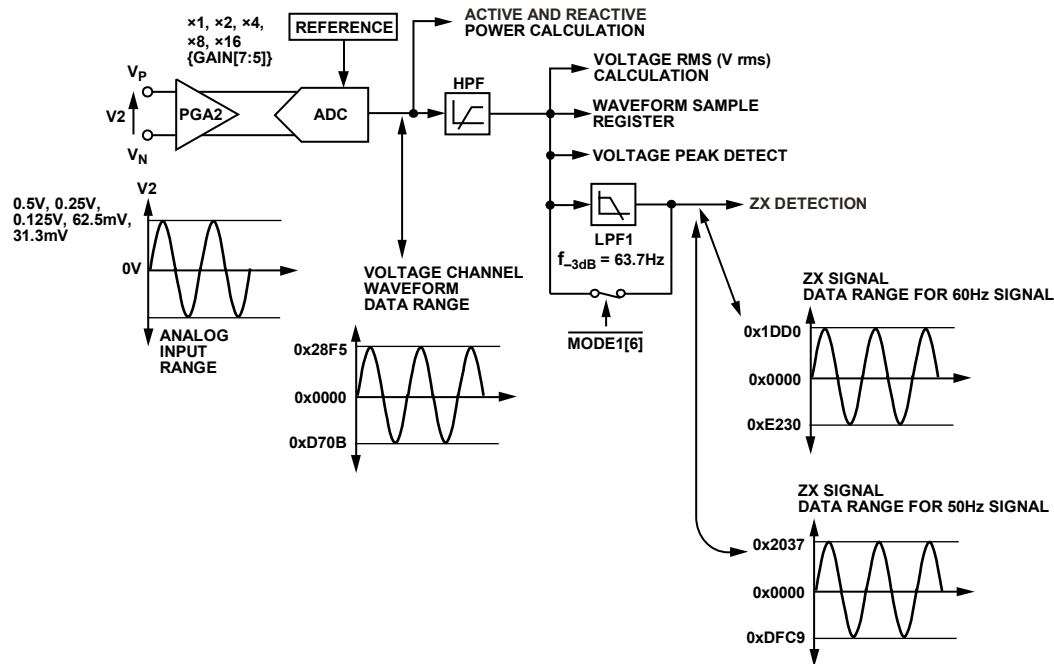
Figure 36. ADC and Signal Processing in Voltage Channel
