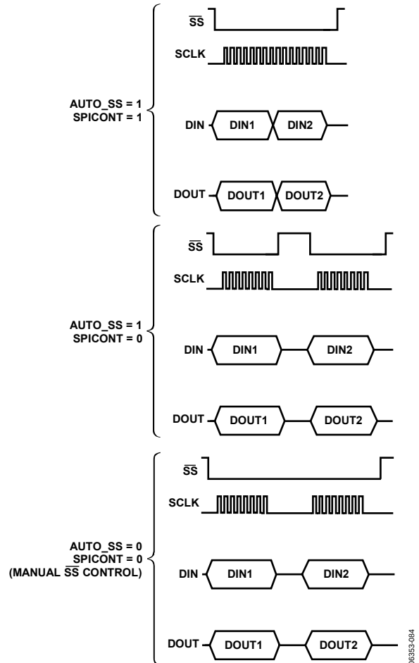
Figure 95. Automatic Chip Select and Continuous Mode Output
