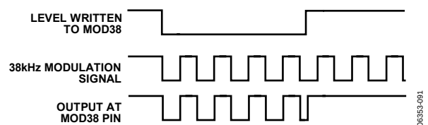
Figure 102. 38 kHz Modulation
