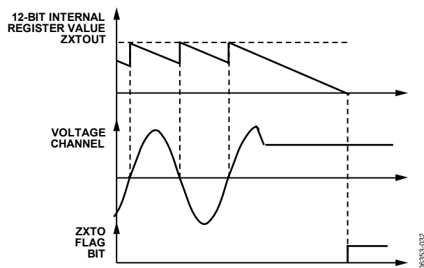
Figure 43. Zero-Crossing Timeout Detection
