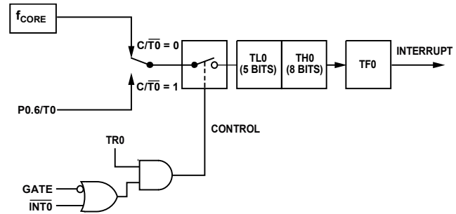
Figure 82. Timer/Counter 0, Mode 0
