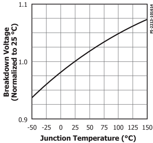
Figure 18. Breakdown vs. Temperature.
