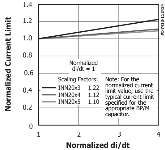
Figure 19. Standard Current Limit Vs. di/dt.
