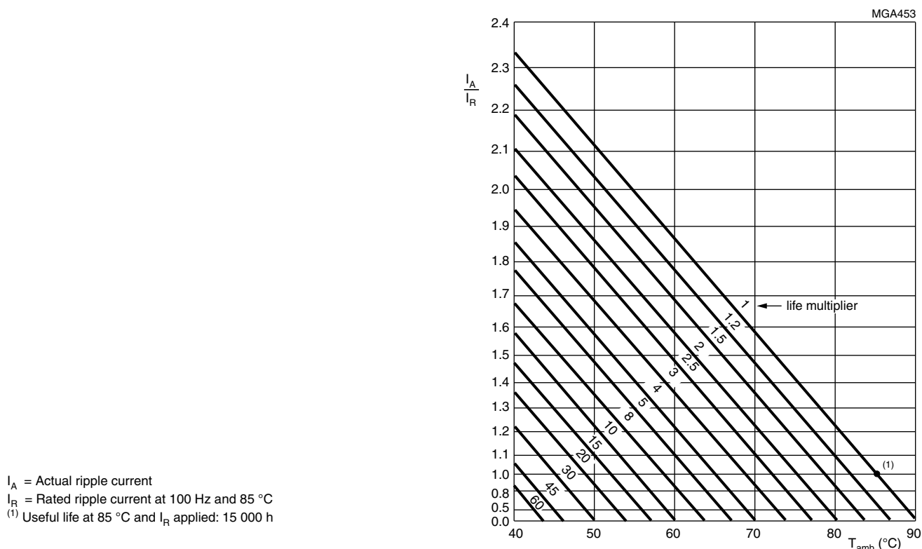
Fig. 29 - Multiplier of useful life as a function of ambient temperature and ripple current load
