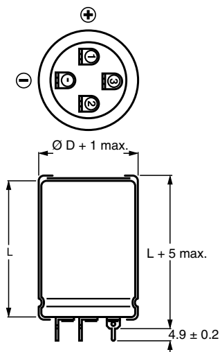
Case Ø D = 30 mm
