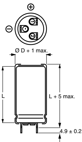
Case Ø D = 25 mm
