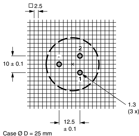
Fig. 3 - Mounting hole diagram viewed from component side
