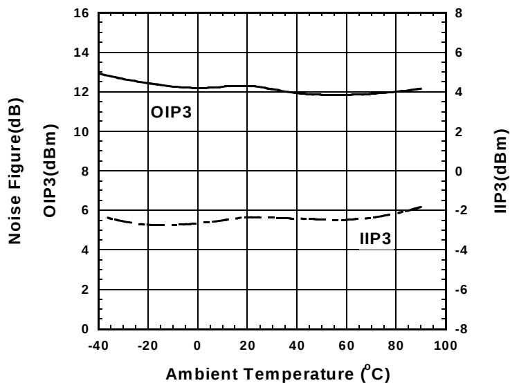
OIP3, IIP3 vs. Temperature
