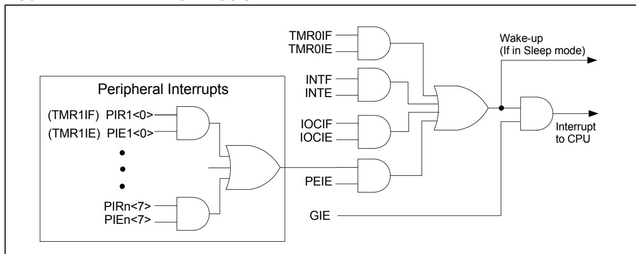
FIGURE 7-1: INTERRUPT LOGIC
