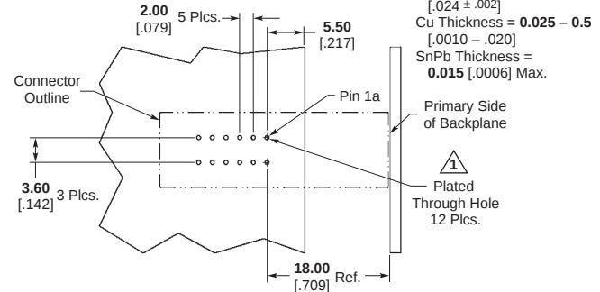
Recommended PCB Hole Layout
