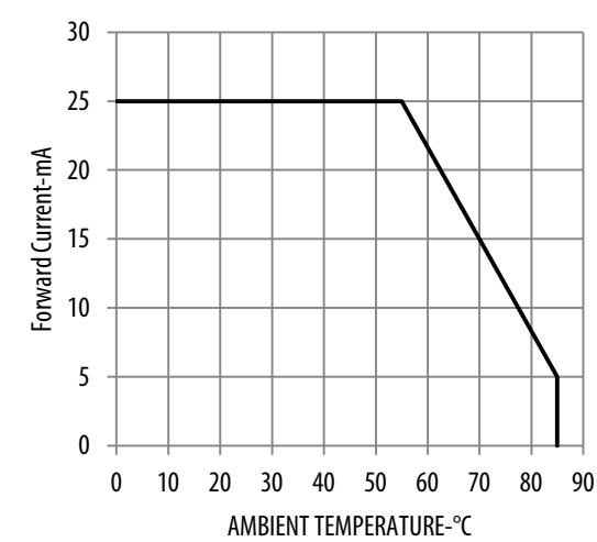
Figure 10: Derating Curve
