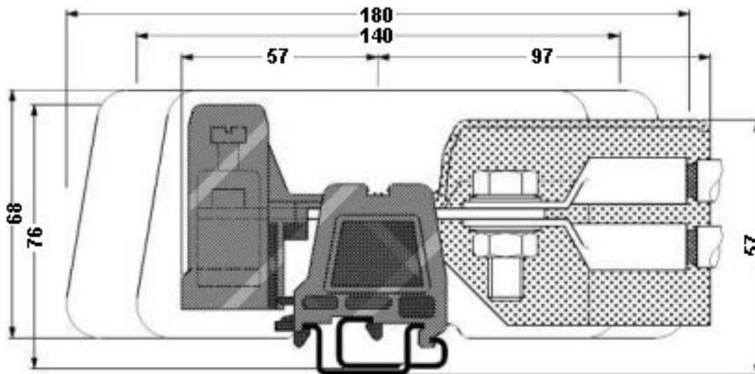
Dimensioned drawing
