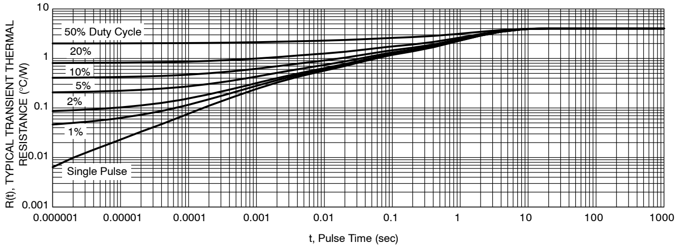
Figure 8. Typical Transient Thermal Response for NTSJ20120CTG
