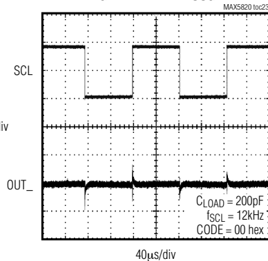
DIGITAL FEEDTHROUGH
