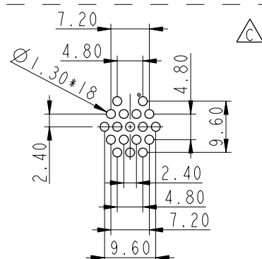
18 Pin Male Connector Male Pin PCB Layout
