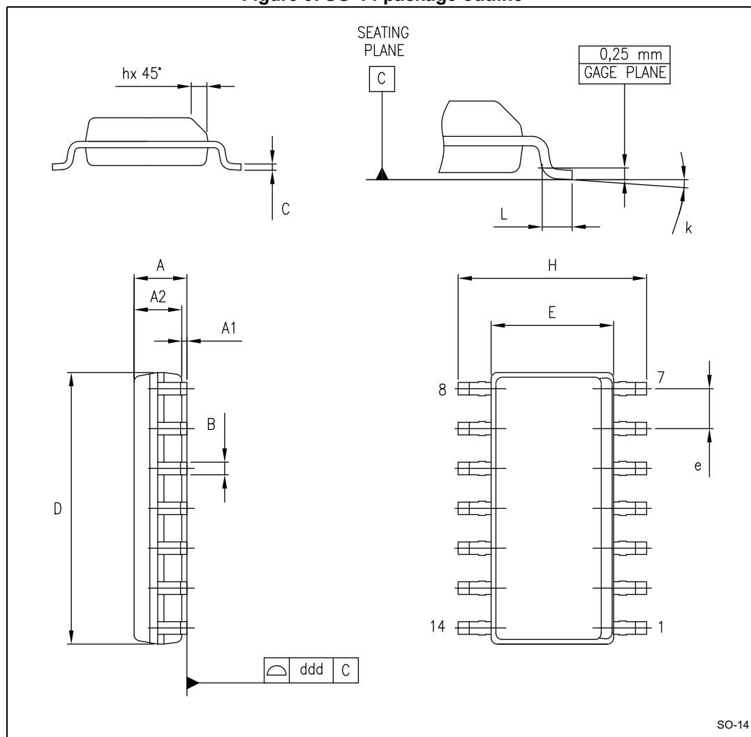
Figure 9. SO-14 package outline
