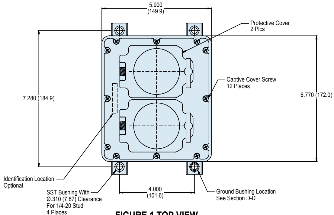
FIGURE 1 TOP VIEW
