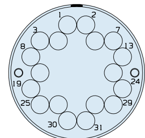
Shell Size 23-18
