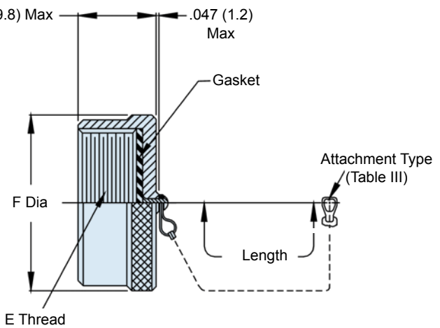
660-073 Receptacle Cover MIL-PRF-28876/15 Style
