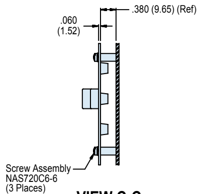
VIEW C-C
