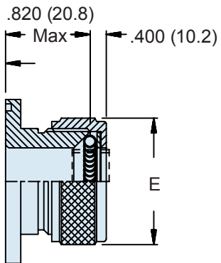
Style 1 Front Mount Type B RFI/EMI (Shown With Style G Gland Nut)
