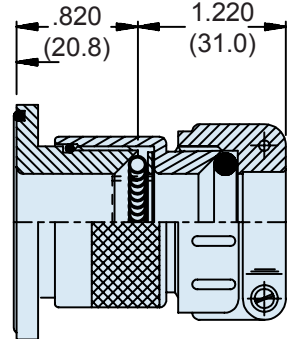
Style 2 Front Mount Type B RFI/EMI Environmental (Shown With Style F Strain Relief)
