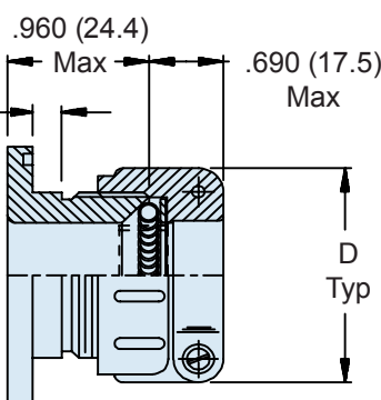
Style 1 Rear Mount Type A RFI/EMI (Shown With Style F Strain Relief)
