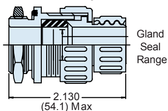
Style E Environmental Conduit Adapter
