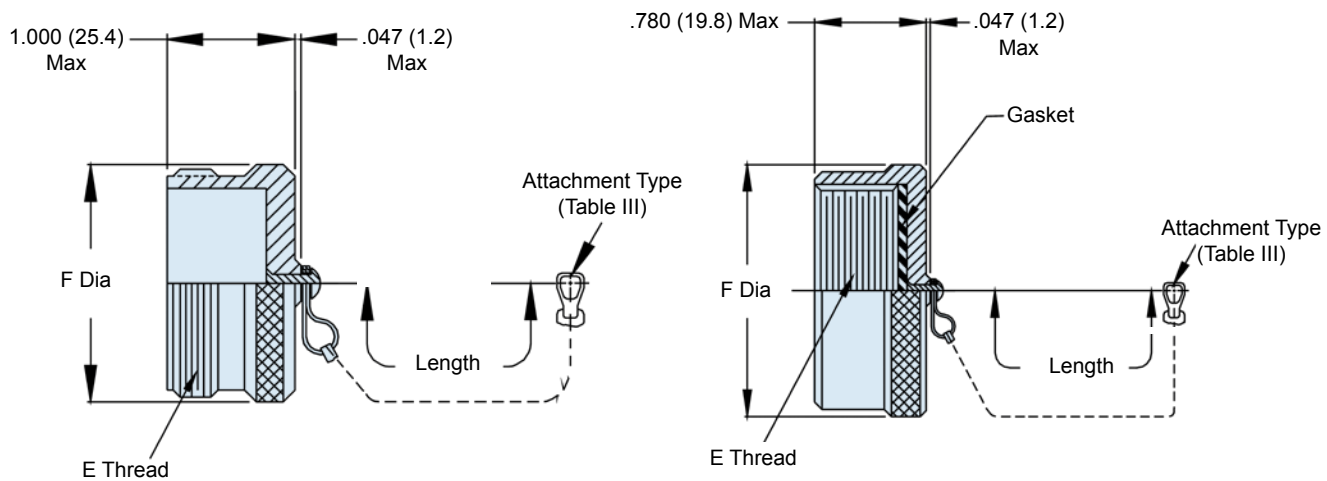
660-072 Plug Cover MIL-PRF-28876/10 Style
