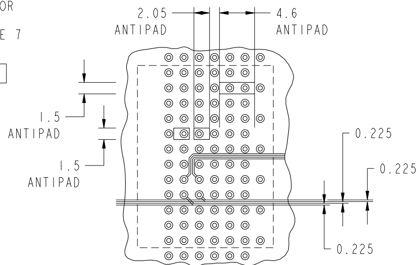
RECOMMENDED TRACK AND ANTIPAD DIMENSIONS SCALE 2:1
