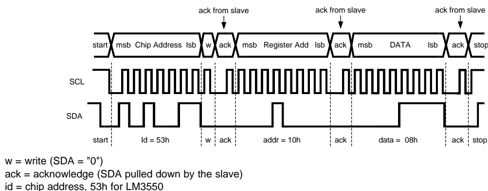
Figure 51. Write Cycle
