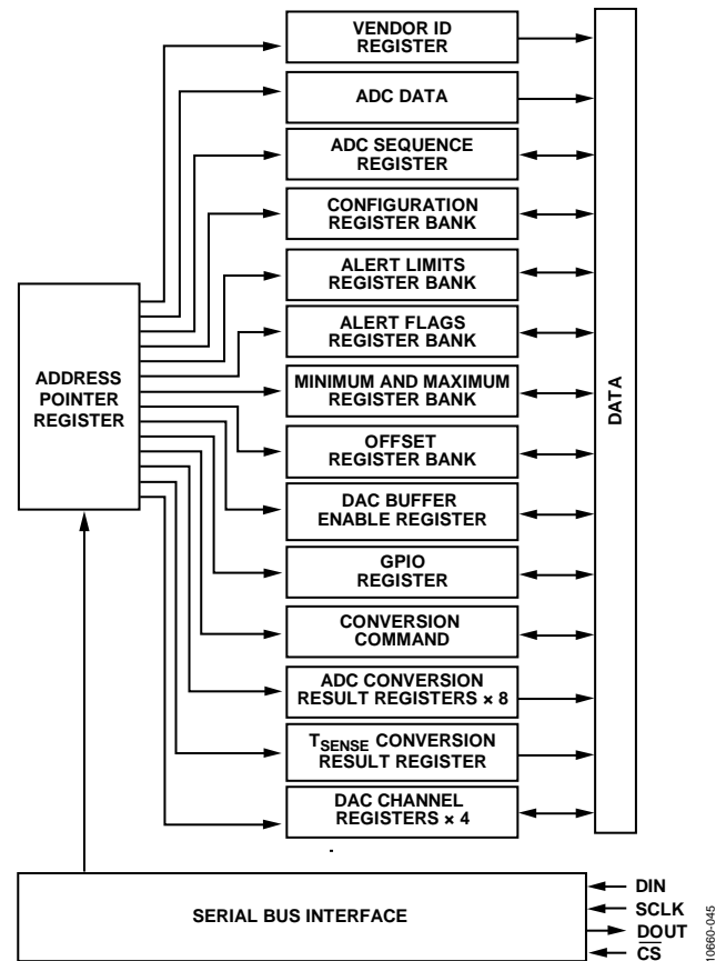
Figure 39. AD7292 Register Structure
