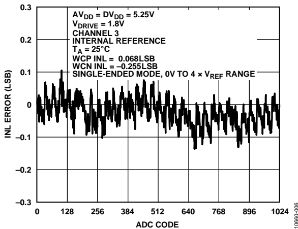
Figure 5. Typical ADC INL, Single-Ended Mode
