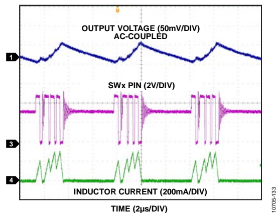
Figure 29. Typical PSM Operation, V_{OUT} = 3.3\text{ V} , I_{LOAD} = 50\text{ mA} , 150\text{ mA}
